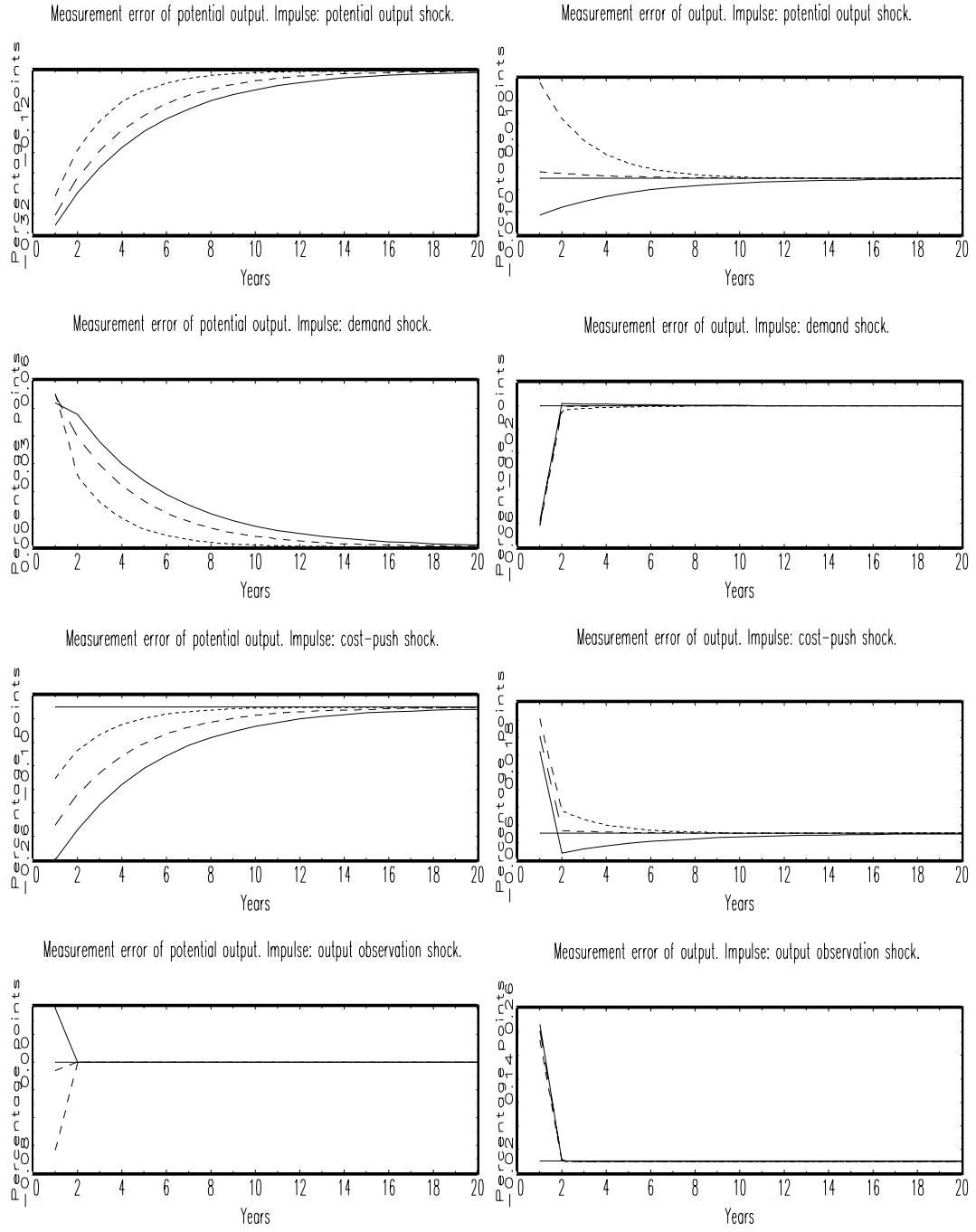
Figure 3: Perception errors.
