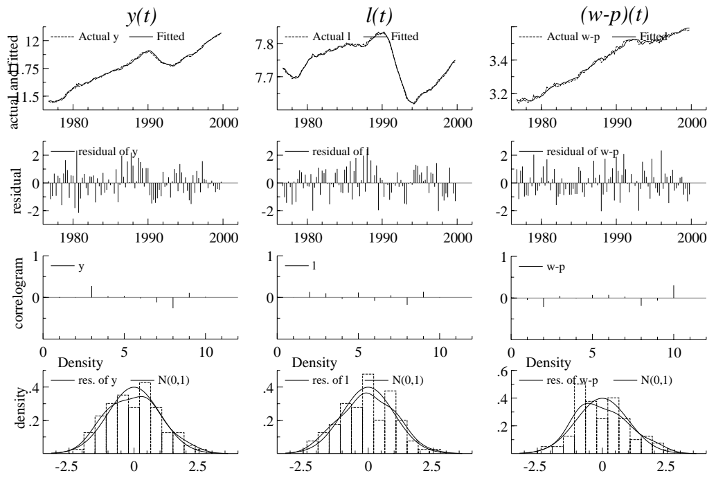
Figure 4 Residual diagnostics
