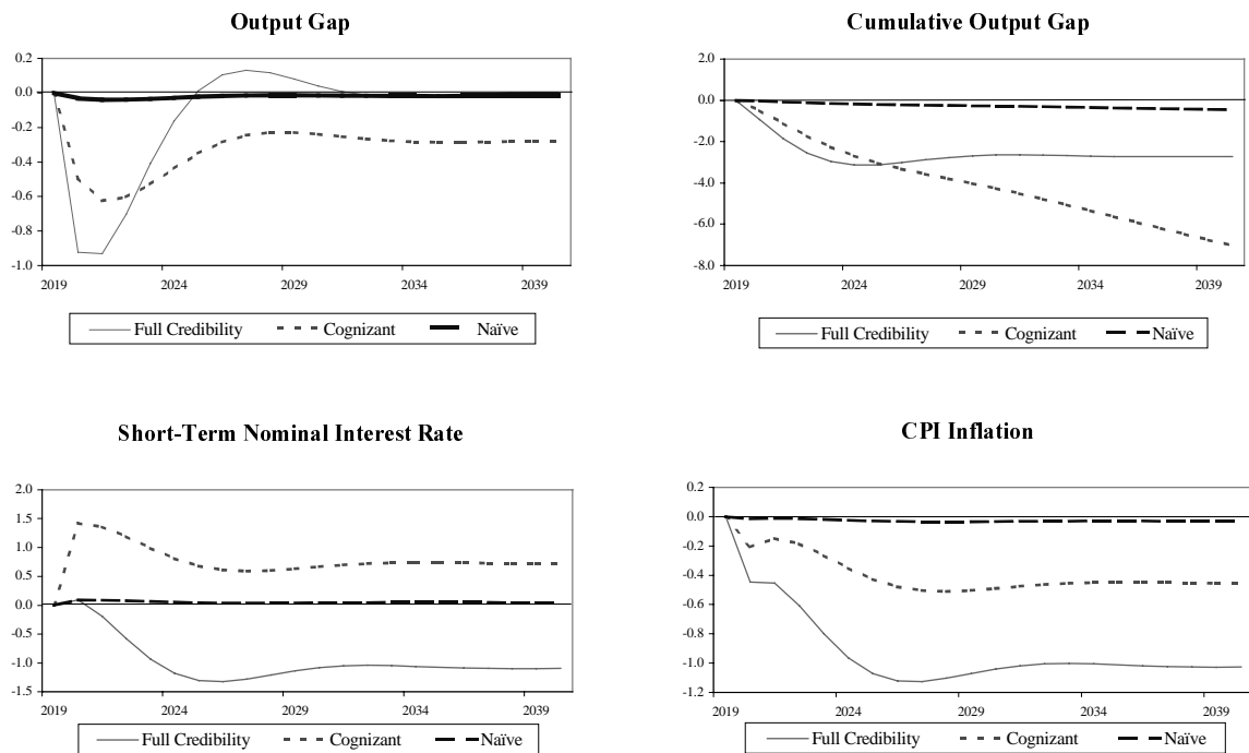
Figure 1: MULTIMOD replication of the disinflation simulations
