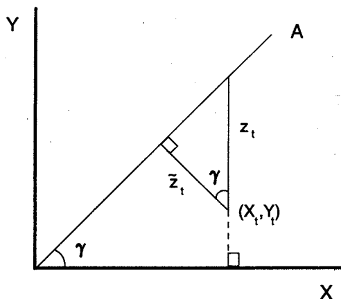
Figure 1. An attractor
