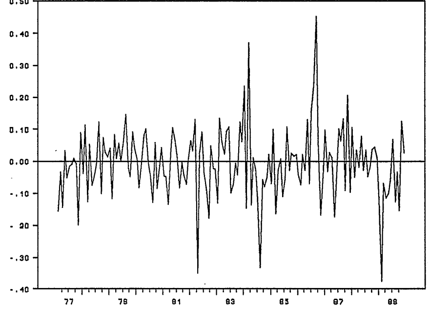
Sample Two, Kalman Filter AR1 Estimation for Beta Series
