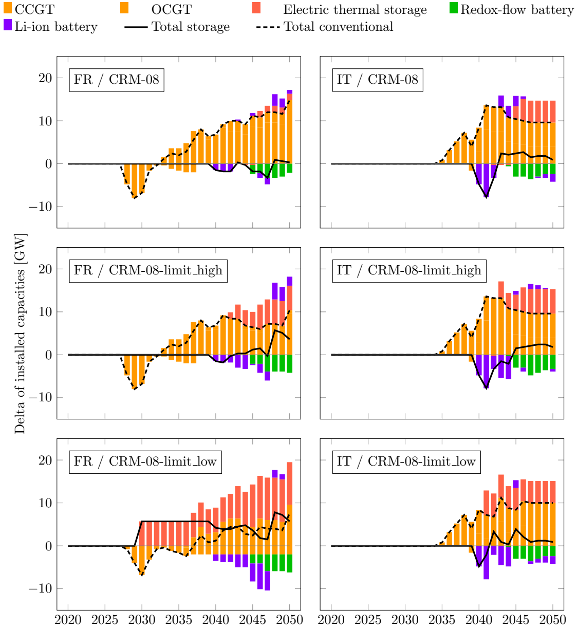
Figure 8: Simulated development of the conventional power plant and utility-scale storage capacities in France (left) and Italy (right) under capacity remuneration mechanisms with different strike prices (from top to bottom: none, high, low). The values shown are the respective deltas of installed capacities as compared to the European energy-only market design.
