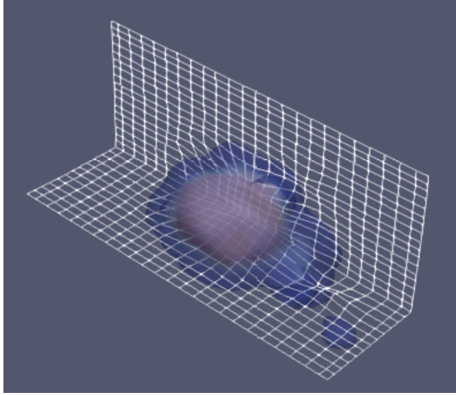
Figure 2: Graphical representation of the nonlinear factors. Colored surfaces show contours of constant estimated density of the data generating process while the grids represent the 3 most important nonlinear factors as a curvilinear coordinate system (L-shaped cross-section shown, for clarity). Both objects are three dimensional cross sections of four dimensional quantities, for plotting purposes. The underlying cartesian coordinate system used is defined by the four most important linear PCA components (with the 4th component not shown here).
