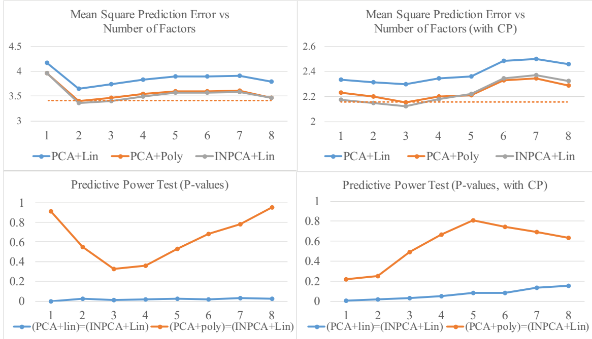
Figure 3: Top panels: Excess bond returns prediction errors for the different models considered in the text as a function of the number of factors included. Bottom panels: Corresponding p -values of tests that the expected squared prediction errors of the various models are equal, as a function of the number of factors included. The right panels report models that include the CP factor while the left panels report those that exclude it.
