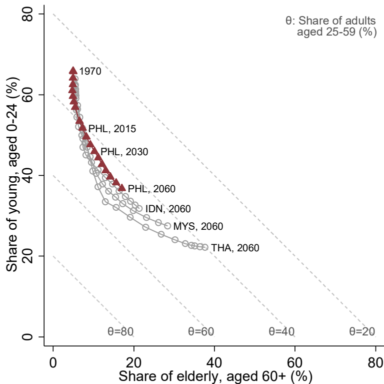
Figure 1. Population age distribution: Selected countries, 1970-2060
