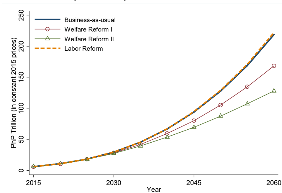
Figure 8. Projected Public Debt, 2015-2060
