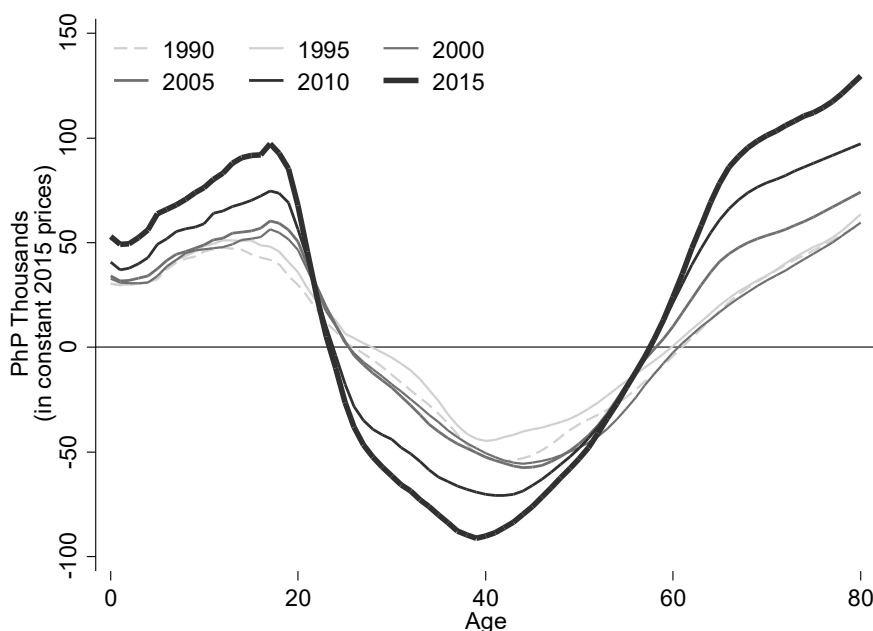
Figure 4. Lifecycle deficit per capita age profile: Philippines, 1990-2015
