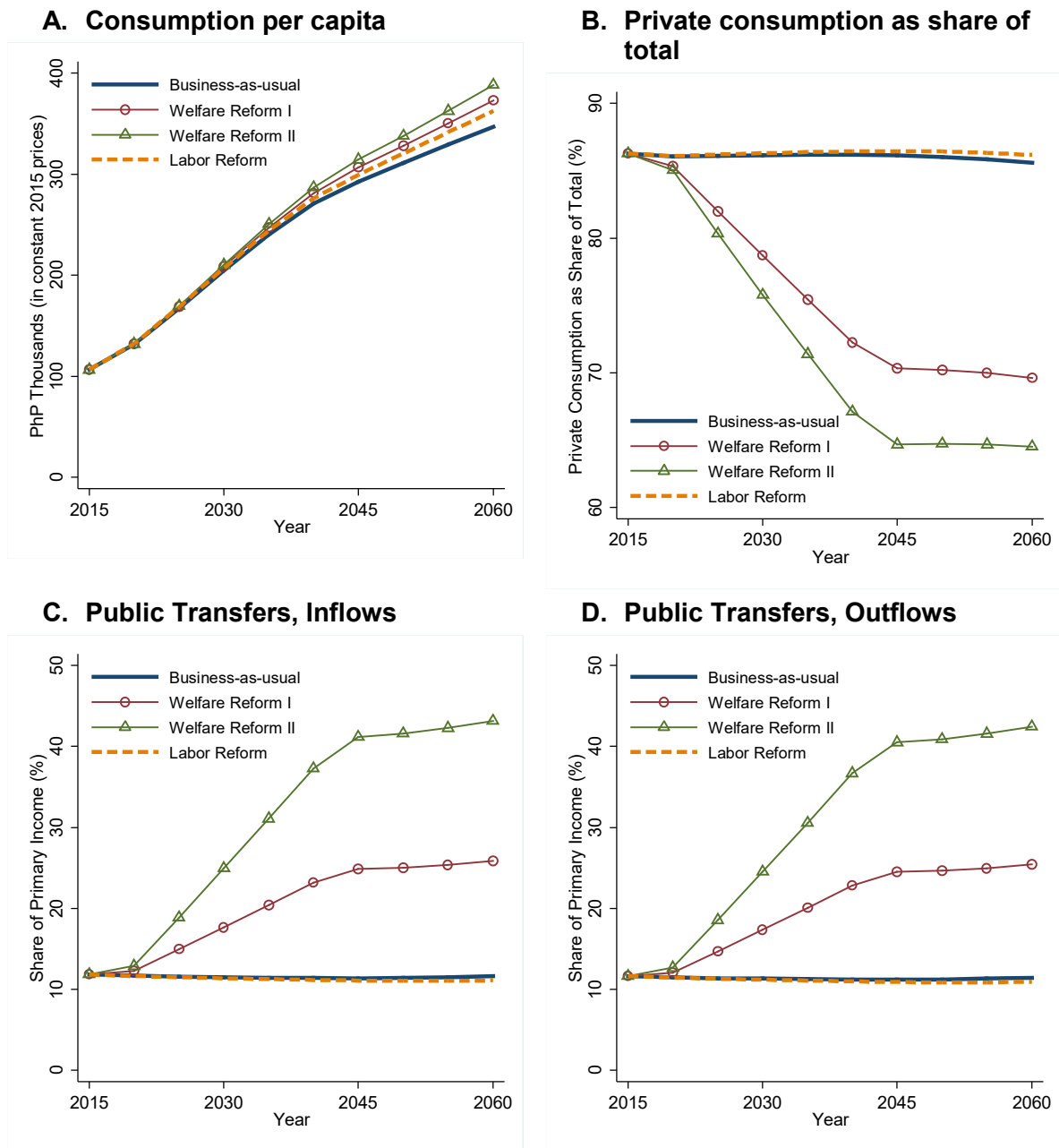
Figure 7. Projected Consumption and Public Transfers, 2015-2060
