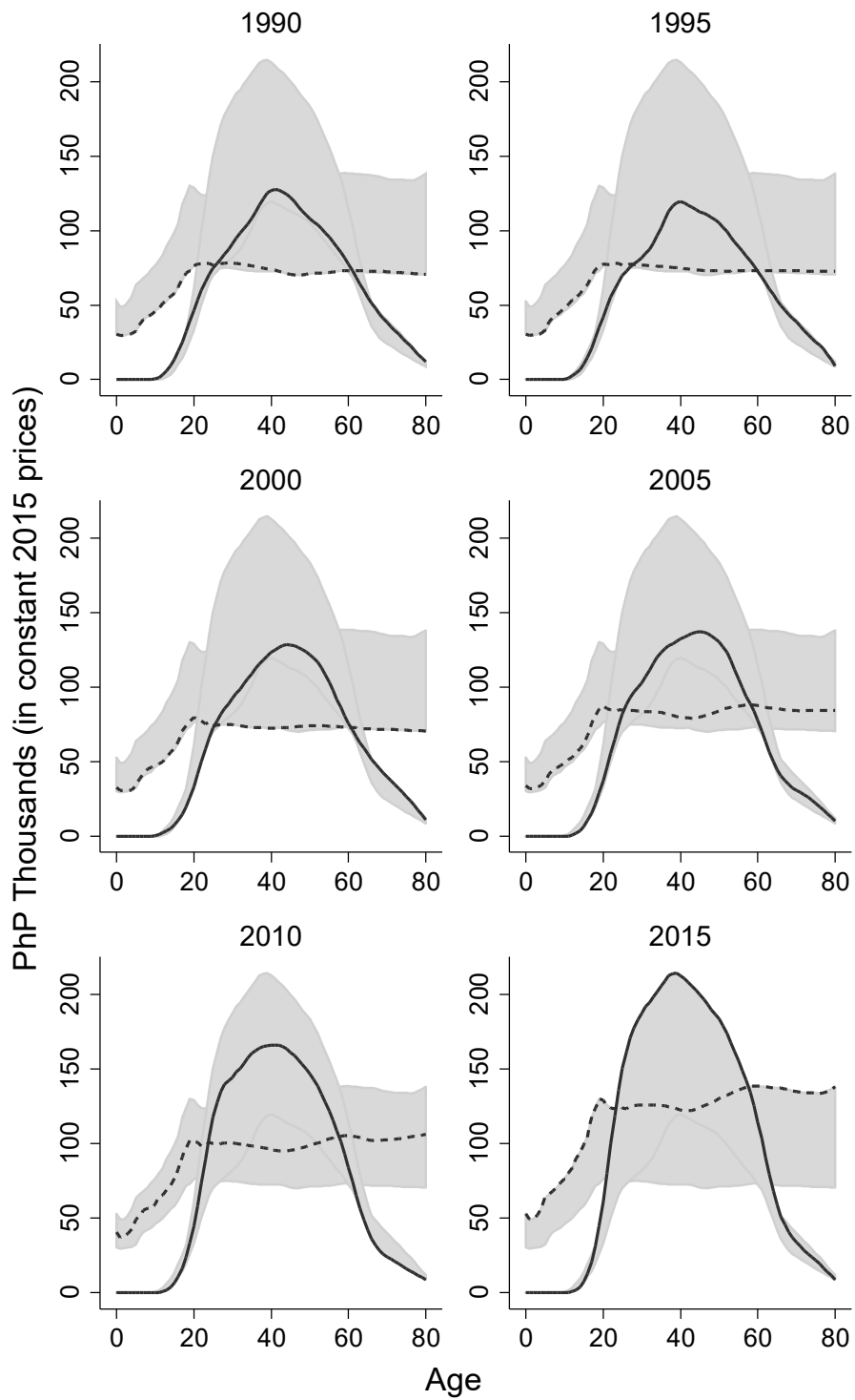
Figure 3. Per capita age profiles of labor income and consumption: Philippines, 1990-2015
