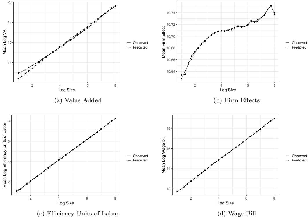
Figure 4: Fit of the Model for Untargeted Moments
