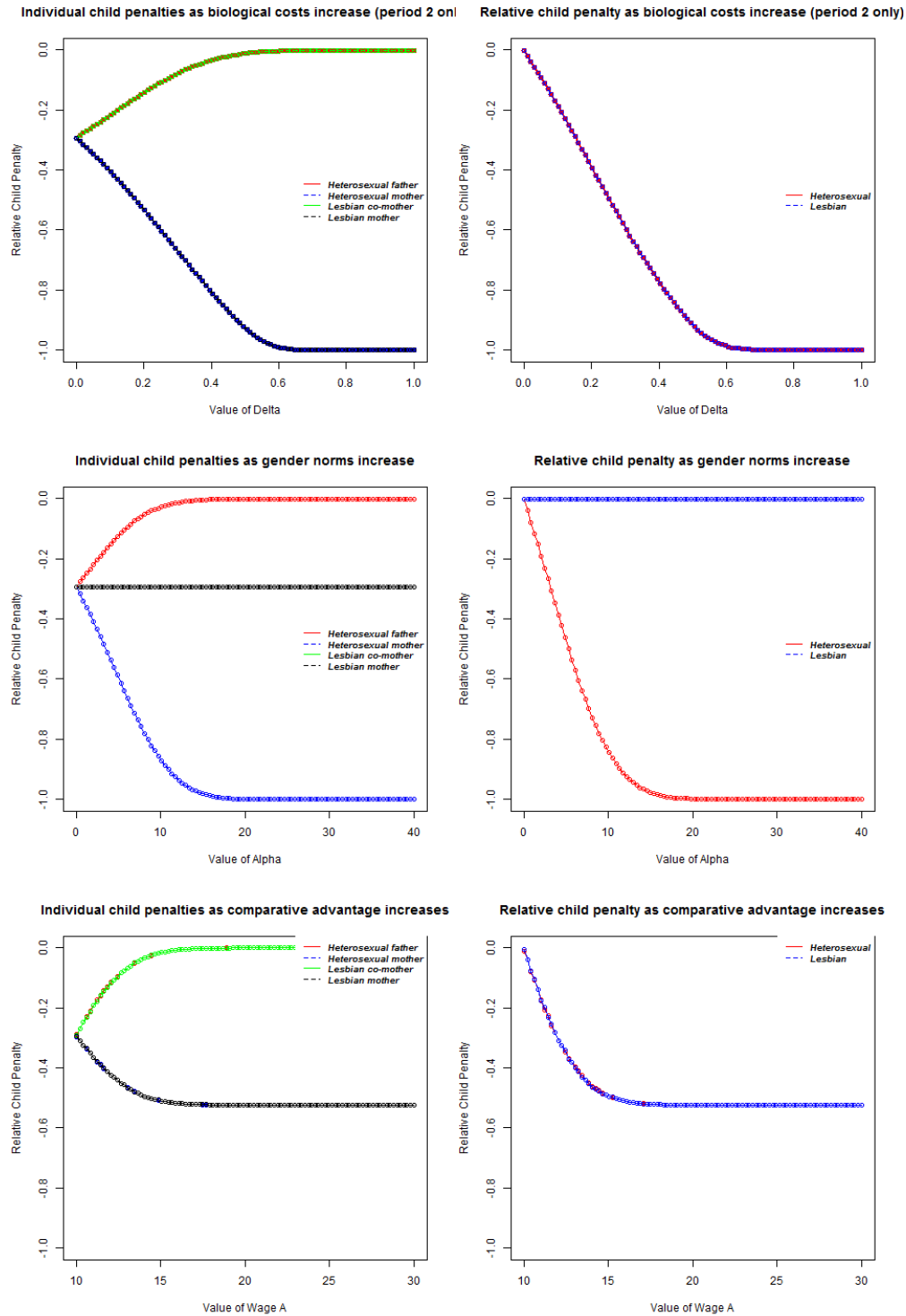
Figure A1: Model Predictions: Simulations for Gender Norms and Specialization
