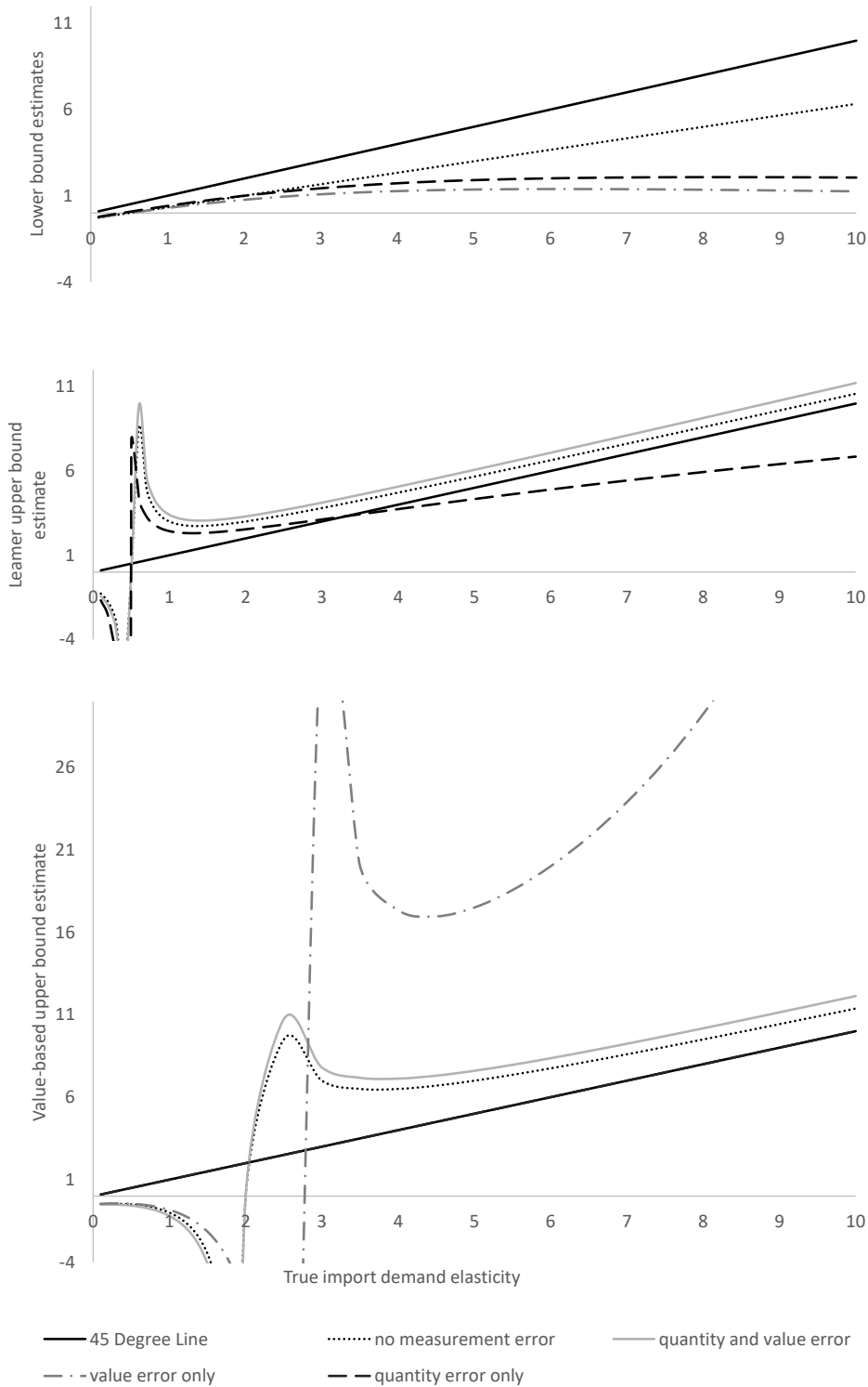
Figure 2: Theoretically predicted lower and upper bounds with measurement error. Notes: \gamma = 1, \sigma_\varepsilon^2/\sigma_\eta^2 = 0.5 in all cases. \sigma_u^2/\sigma_\eta^2 = 0, \sigma_w^2/\sigma_\eta^2 = 0.05 in quantity measurement error case. \sigma_u^2/\sigma_\eta^2 = 0.05, \sigma_w^2/\sigma_\eta^2 = 0 in value measurement error case. \sigma_u^2/\sigma_\eta^2 = \sigma_w^2/\sigma_\eta^2 = \sigma_{uw}/\sigma_\eta^2 = 0.05 in quantity and value error case. Source: authors' calculations
