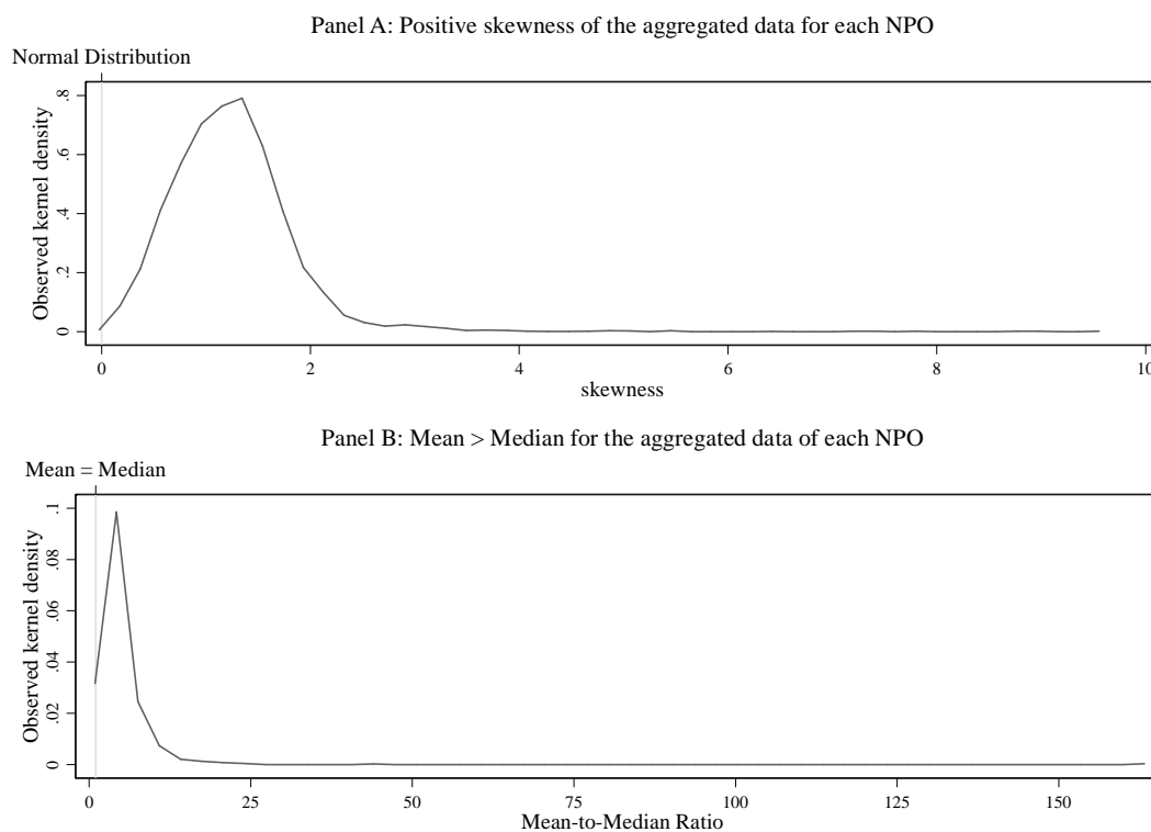
Figure A1. Distribution of skewness and mean-to-median ratio of the aggregated data
