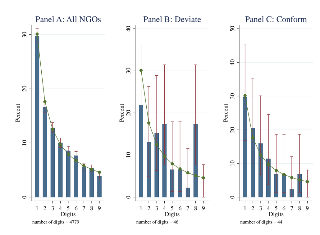
Figure 2. The Ugandan NGO financial data and conformity to Benford's Law
