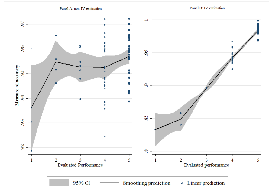
Figure A4. Semiparametric non-IV and IV estimation following Robison (1988) selection model.
