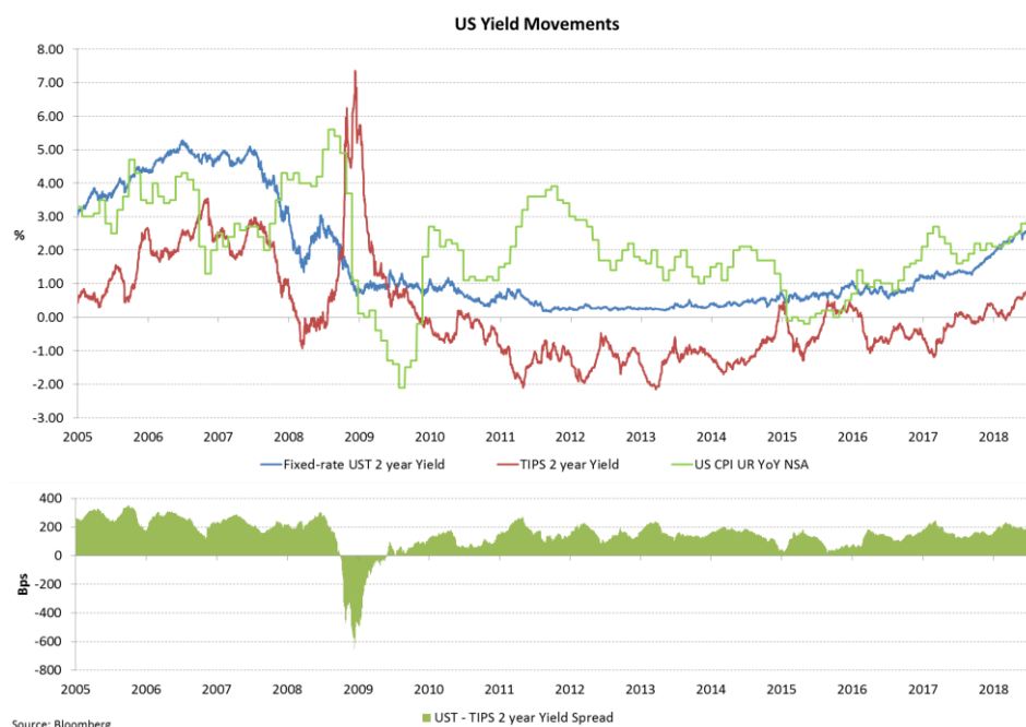
Figure 5: US fixed rate and inflation-linked bonds yields and realised inflation.
