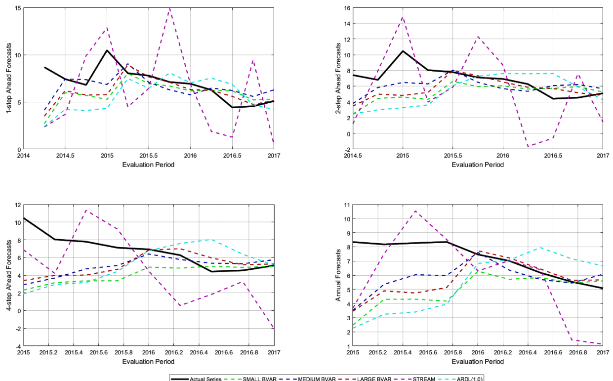
Figure 1: GDP forecast evaluation at different projection horizons (percentage changes)
