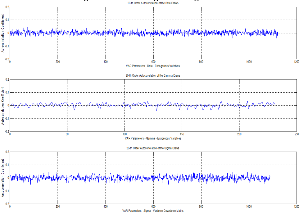
Figure A4: Convergence Diagnostics
