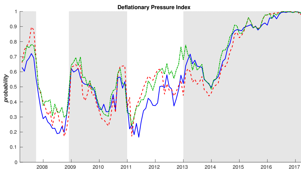
Figure 8: Deflationary pressure index. This is the simple average of the out-of-sample forecasts for all horizons. AUROC (solid blue line), MAE (dash-dot green line), RMSE (dotted red line) highlight the index made from models selected independently with these three criteria. The gray bars represent periods with inflation smaller than 2%.
