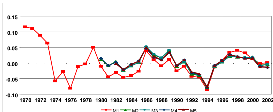
CHART 4.7: RESIDUAL PLOT
