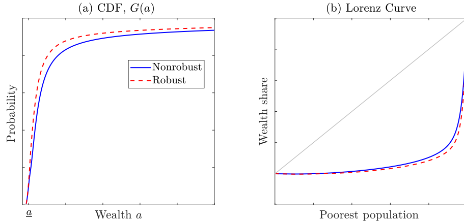
Figure 3: Distributional statistics
