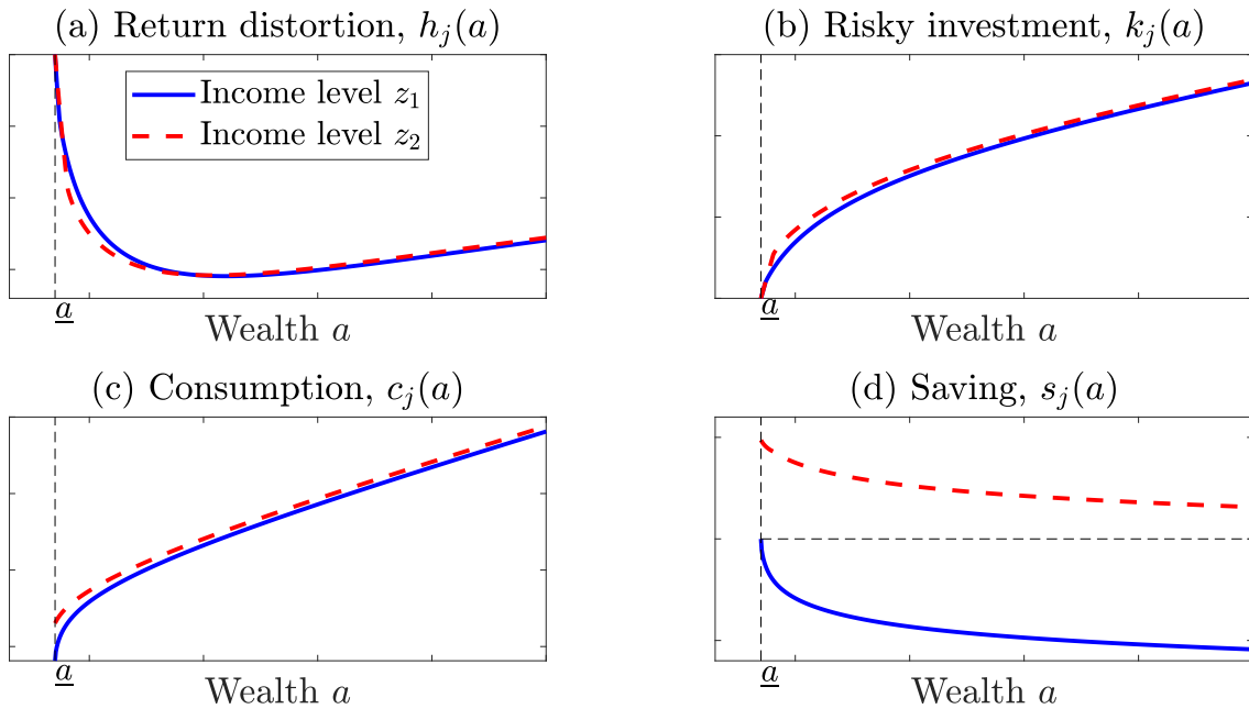
Figure 1: Policy functions
