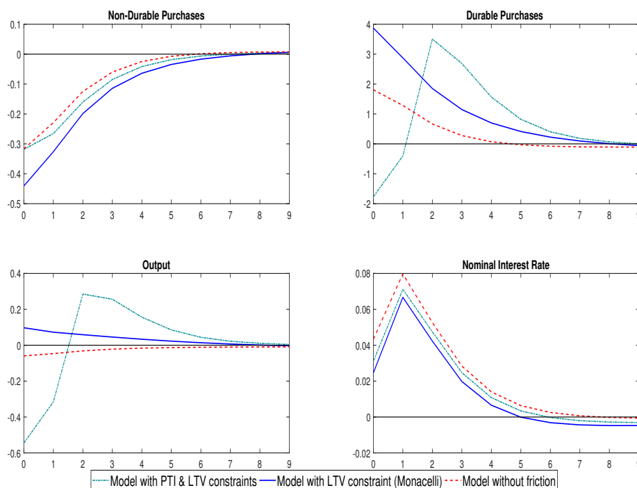
Figure 3 Comparison of the models: two frictions, one friction, and no frictions, at fully flexible durable prices
