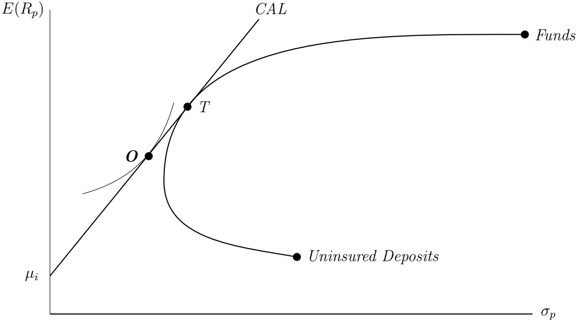
Figure A1: The household's optimal three asset portfolio decision when the "quantity constraint" is not binding
