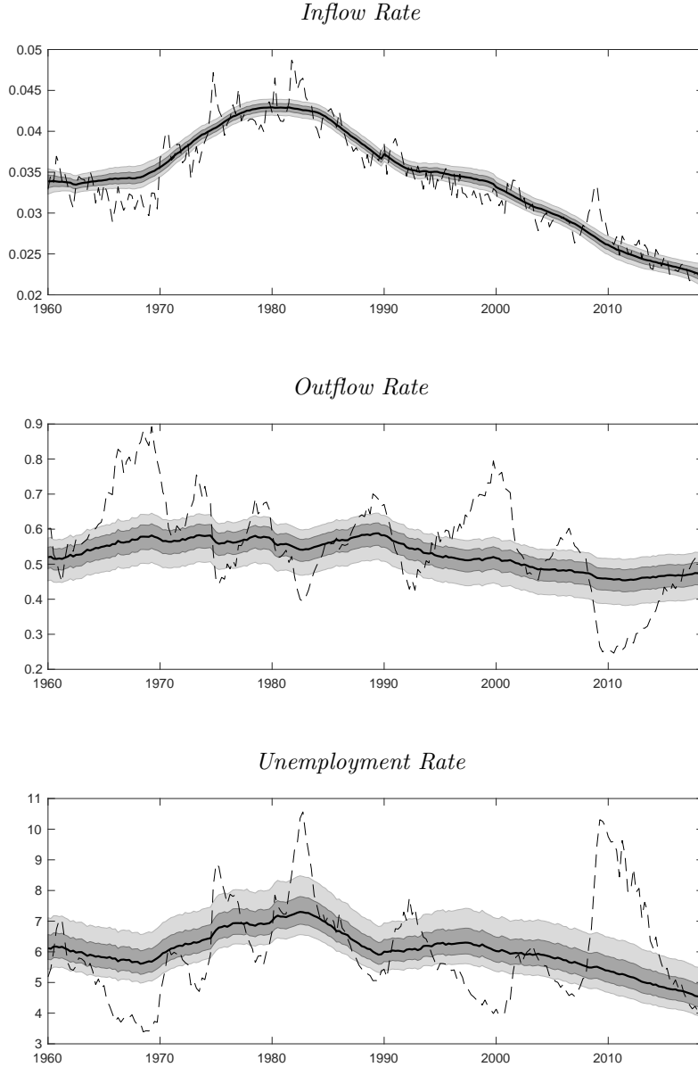
Figure 6. Inflow rate, outflow rate and unemployment rate along with estimated secular trend Actual rates denoted by dashed lines, median estimates of secular trend ( \bar{s}_t , \bar{f}_t , and \bar{u}_t ) denoted by solid black lines. Shading denotes 68% and 95% coverage intervals.
