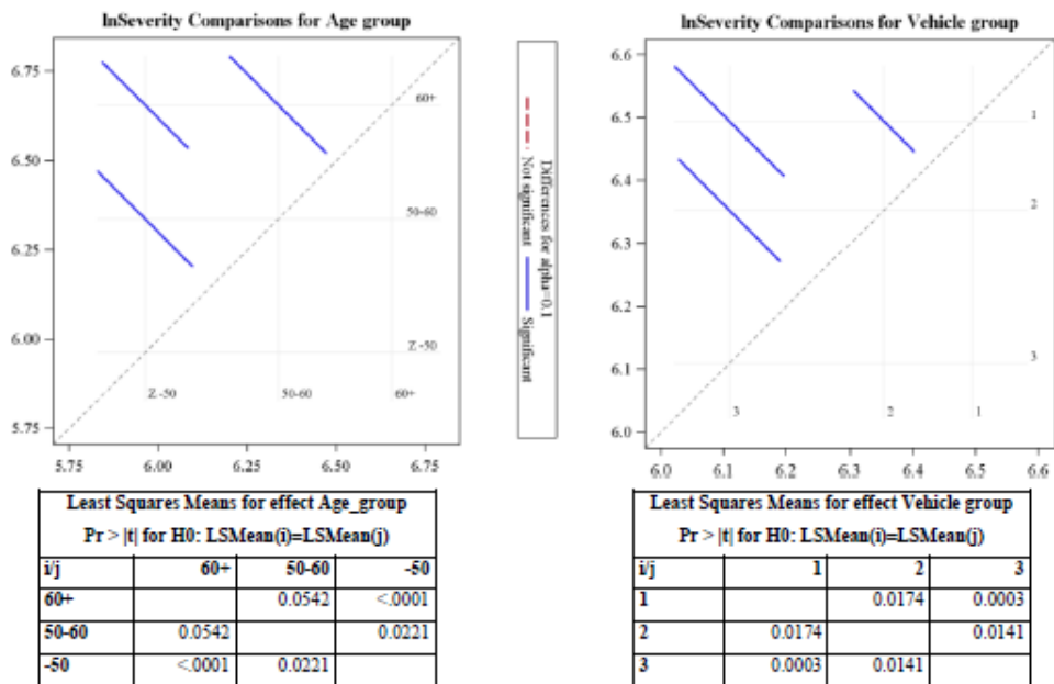
Figure 4. Comparison of LS means for factor Age_group (on the left) and for factor Vehicle group (on the right)
