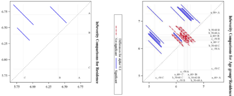
Figure 5. Comparison of LS means for factor Residence (on the left) and for interaction Age_group×Residence (on the right)
