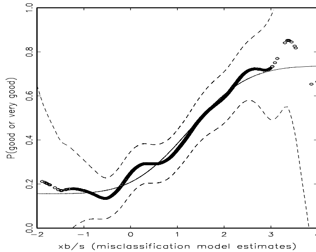
Figure 4. Test of Parametric Misclassification Model
