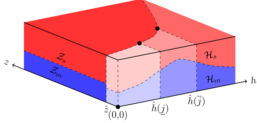
Fig. 7: Equilibrium
