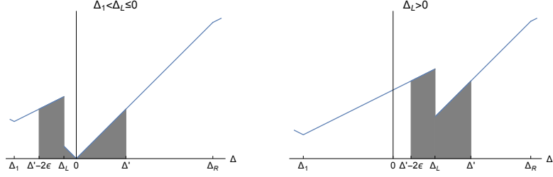
Figure 4: HS1 default ( \bar{\Delta}(\alpha, b, c, \epsilon) = \Delta' ). The shaded area equals \Psi(\alpha, b, c, \epsilon) .
