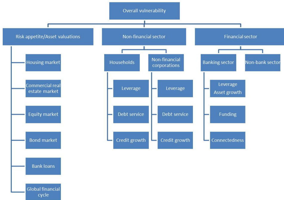
Figure 1: Structure of Heatmap
