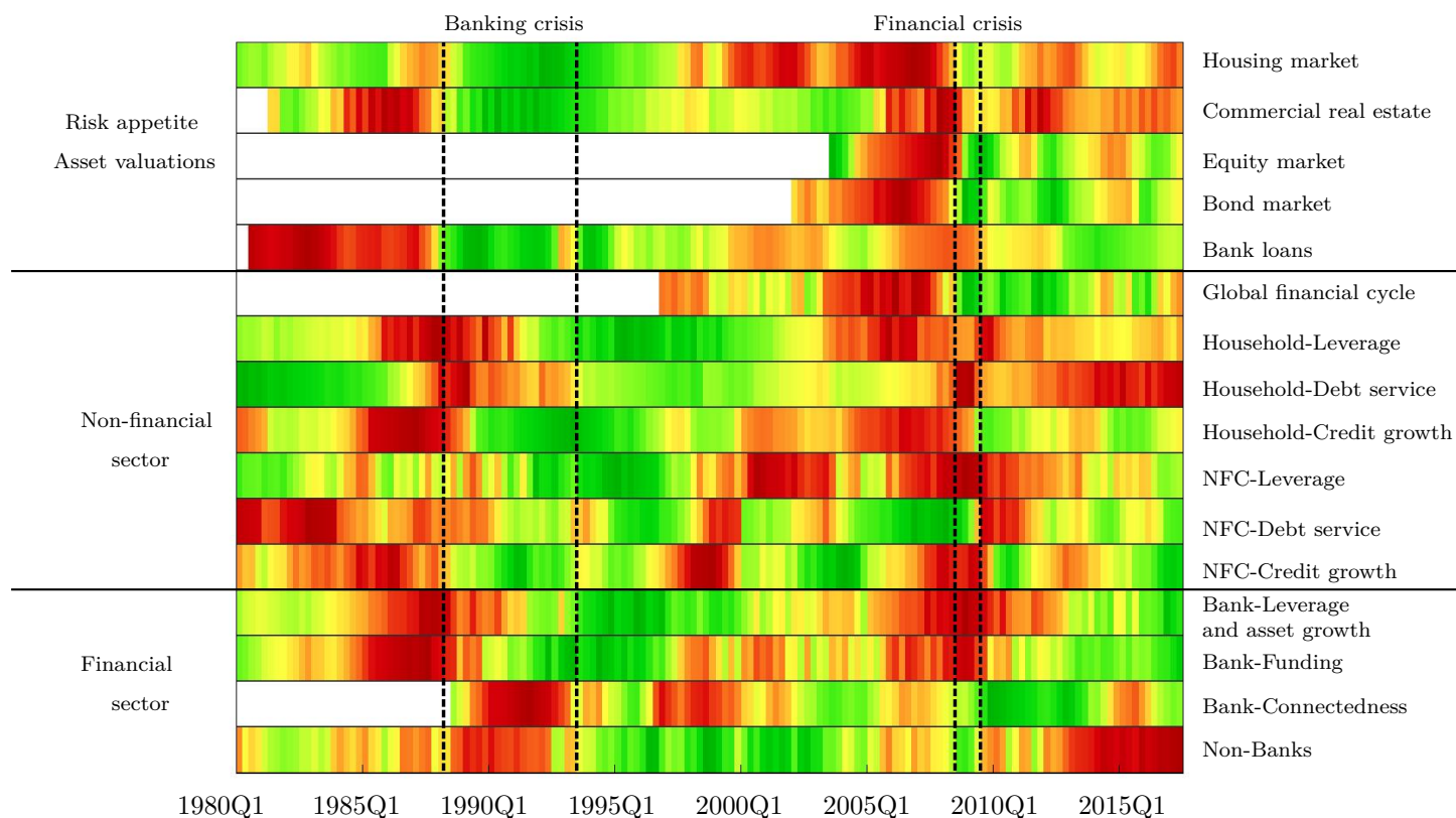
Figure 10: Summary heatmap: Non-recursive 1980Q1-2017Q2
