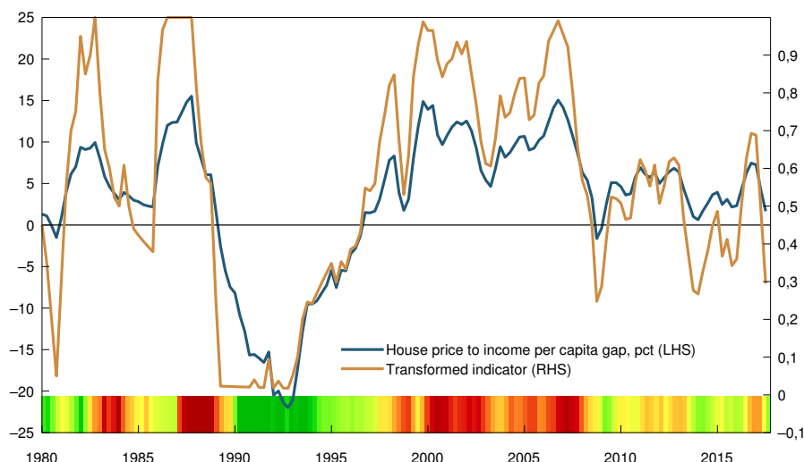
Figure 6: Data transformation: An example using house price to disposable income per capita gap (recursive)
