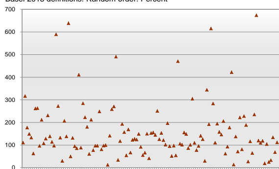
Chart 25. LCR for all Norwegian banks as of 2014 Q2. Basel 2013 definitions. Random order. Percent
