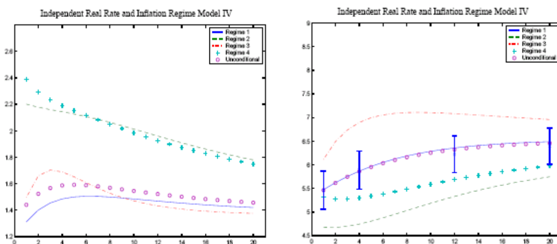
Figure 4.1: Term structure of real (left panel) and nominal (right panel) interest rates under different regimes in a regime shifting model as presented in Ang and Bekaert (2005). Regime 1 has low and stable real rates and high and stable inflation. Regime 2 has high and stable real rates and low and stable inflation. Regime 3 has low and volatile real rates and high and volatile inflation. Regime 4 has high and volatile real rates and low and volatile inflation. Units on the y-axis are percentage and units on the x-axis are maturity in quarters of a year. In the right panel, vertical bars and faint x's in the middle of the bars indicate the standard deviation and historical average of the observed nominal rates Data is CRSP zero coupon rates in USA and seasonally adjusted all urban consumer price inflation, covering the period 1952 to 2000. Source: Copy from figures 3 and 7 in Ang and Bekaert (2005).
