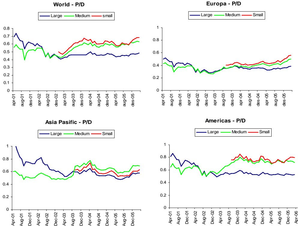
Figure 5.14: FTSE large, mid and small cap index series. Price/dividend ratios
