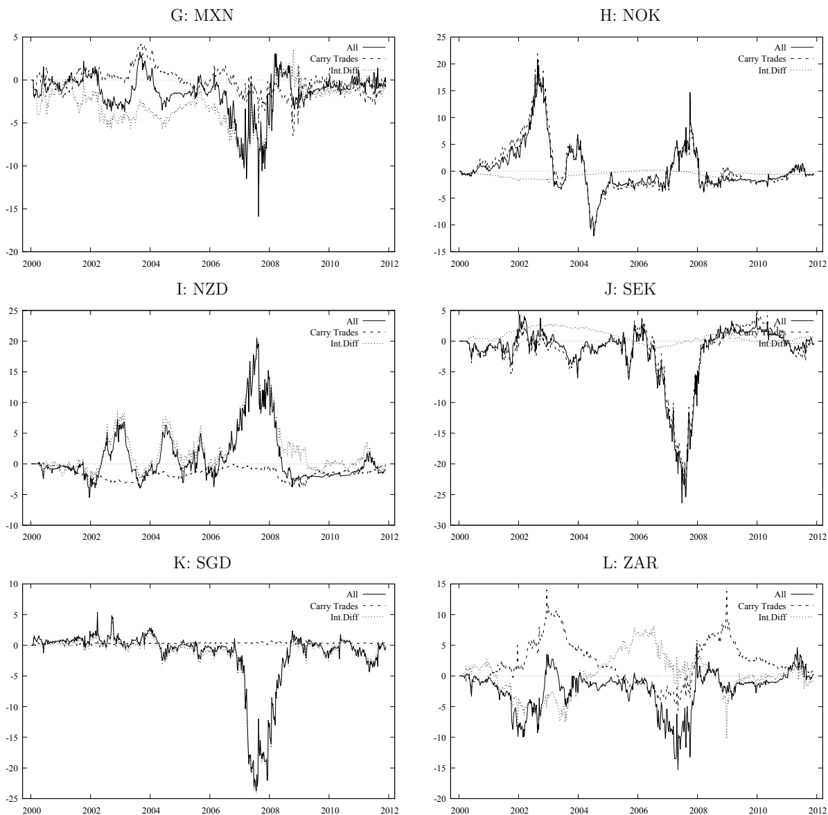
Figure 4: Historical Decompositions for the Carry Trade (Cont.)
