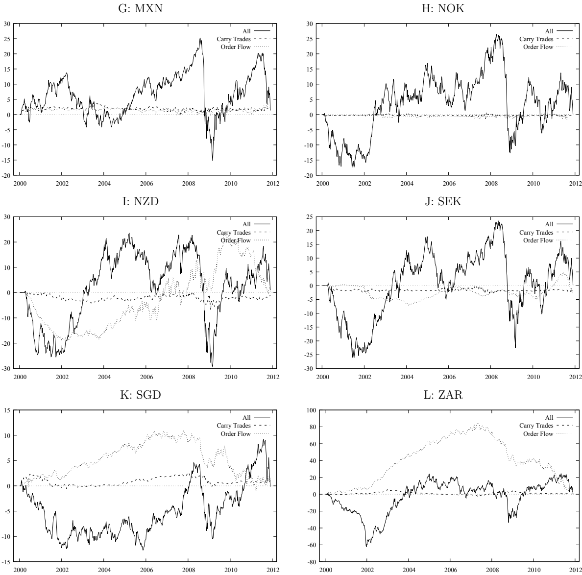
Figure 5: Historical Decompositions for Log Spot Rates (cont.)
