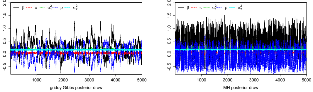
Figure 8: Posterior draws of all parameters for simulated IV data based on the griddy Gibbs sampler and the MH algorithm using MitISEM approximation. Posterior results are obtained as in Table 3.
