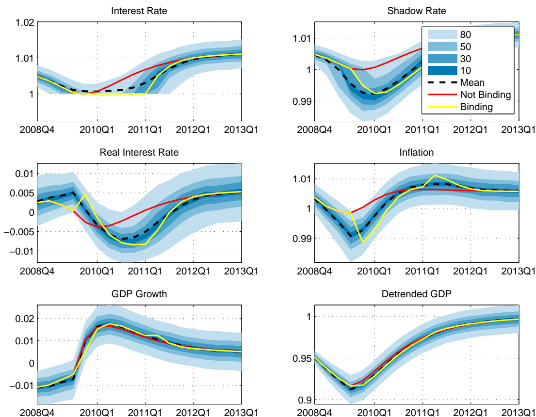
Figure 5: Regime-Switching: Comparison
