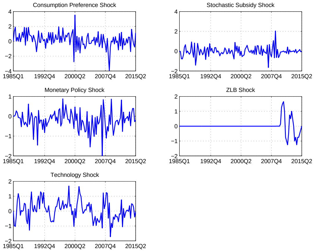
Figure C.16: Model Shocks
