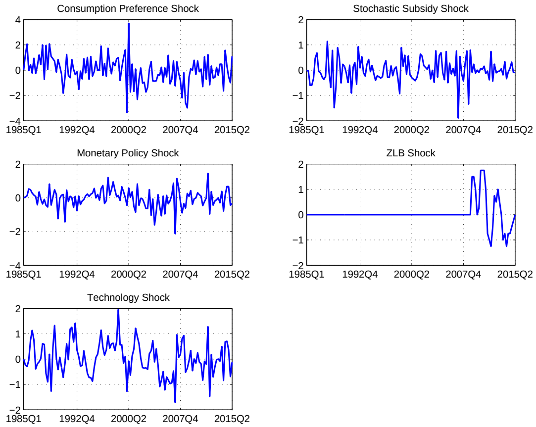
Figure C.19: Model Shocks
