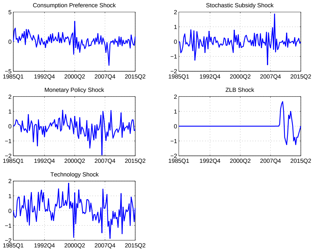
Figure C.14: Model Shocks
