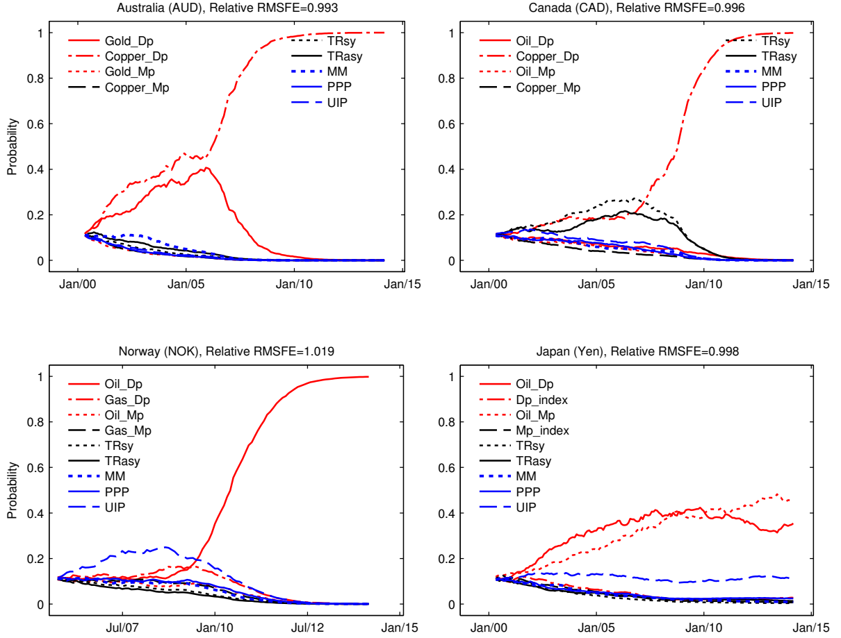
Figure 4: Weights Associated with Each Predictor in the BMA with Daily and Monthly Predictors
