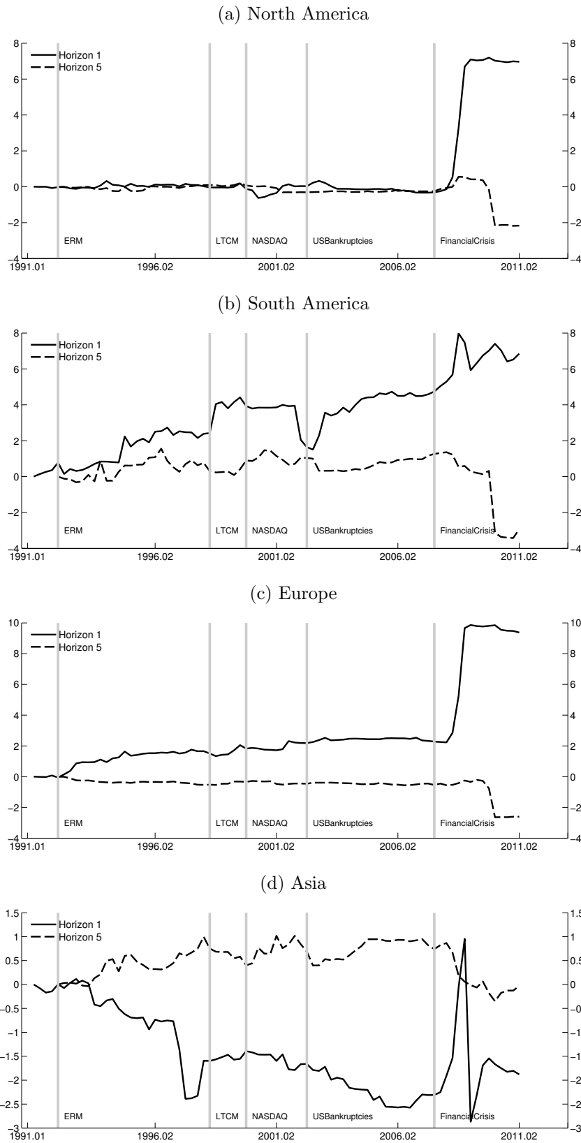
Figure 8: Relative historical forecast performance GDP: Across regions, RMSPE scores
