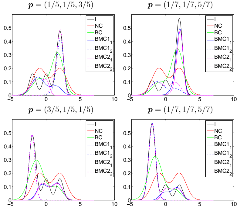
Figure 2: Contribution of the calibration components for different models BC, BMC1 (first and second mixture component, BMC1_1 and BMC1_2 ) and BMC2 (first and second mixture component, BMC2_1 and BMC2_2 ), and different datasets.
