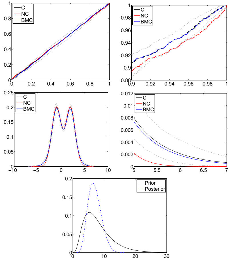
Figure 5: Infinite beta mixture calibrated (BMC), calibrated (C) and non calibrated (NC) combinations for a dataset of 2,000 samples from 1/2\mathcal{T}(-1, 1, 6) + 1/2\mathcal{T}(2, 1, 6) . PITs cdf (top graphs) and calibrated pdf (middle graphs) of the combination models C (black), NC (red) and BMC (blue) and BMC 99% HPD (gray). Prior (black) and posterior (blue) number of components of the random BMC model (bottom).
