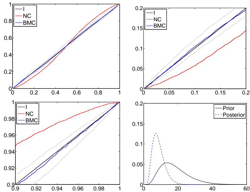
Figure 6: Infinite beta mixture calibrated (BMC), calibrated (C) and non calibrated (NC) combinations for the S&P500 daily percent log returns data. PITs cdf (lines from 1 to 3) of the idea model I C (black), combination models NC (red) and BMC (blue) and BMC 99% HPD (gray). Prior (black) and posterior (blue) number of components of the random BMC model (bottom).
