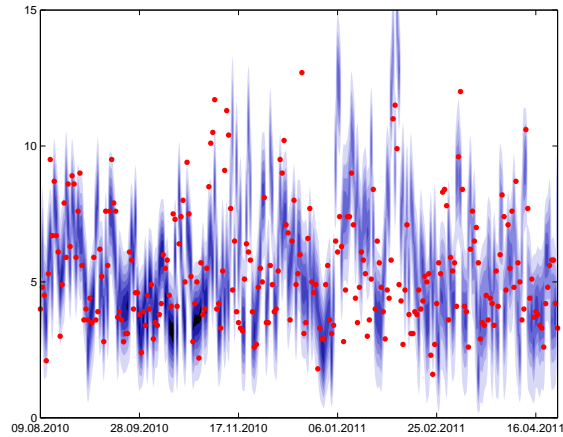
Figure 11: Fanchart of the BMC model and observations (red points) over the sample period from August 9, 2010 to 30 April 2011.
