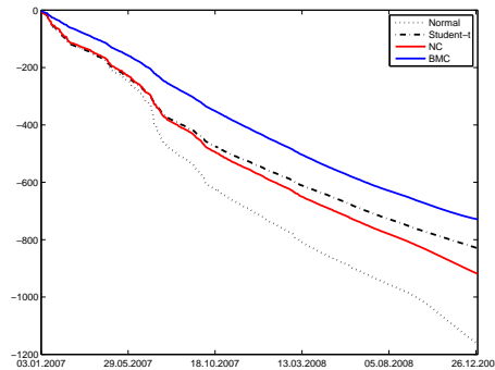
Figure 7: Cumulative log scores for the Normal GARCH model (Normal), t -GARCH model (Student- t ), linear pooling (NC) and beta mixture calibration (BMC) over the sample period from January 1, 2007 to December 31, 2008.
