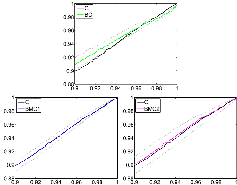
Figure 4: Results of the Bayesian calibration model BC (top), BMC1 (middle) and BMC2 (bottom) for the right tail of the predictive distribution. In each plot the PITs cdf of the calibrated (solid black line) and beta calibrated model (solid coloured line) and their 99% HPD region (gray dashed lines)
