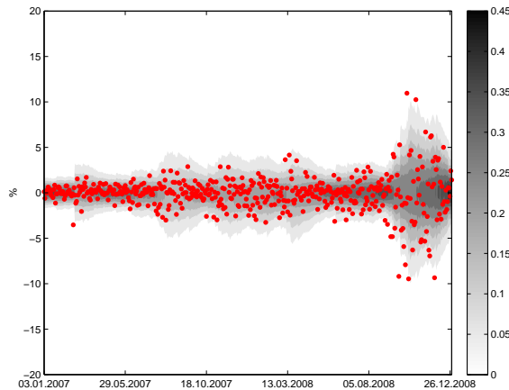
Figure 8: Fanchart of the BMC model and observations (red points) over the sample period from January 1, 2007 to December 31, 2008.
