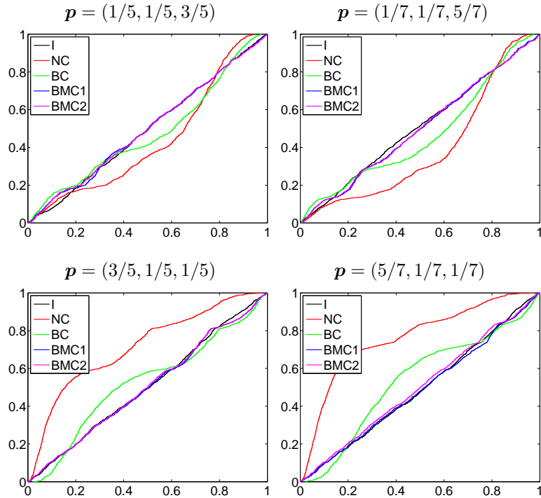
Figure 1: PITs cdf for different calibration models and different datasets.
