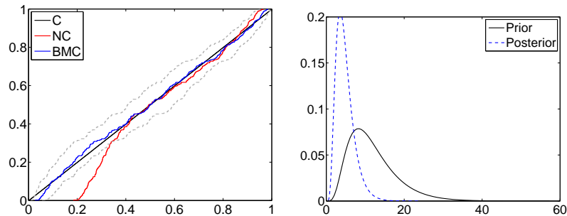
Figure 9: Infinite beta mixture calibrated (BMC), calibrated (C) and non calibrated (NC) combinations for the maximum wind speed at the station at Frankfurt airport. PITs (left top) of the combination models C (black), NC (red) and BMC (blue) and BMC 99% HPD (gray). Prior (black) and posterior (blue) number of components of the random BMC model (right top).
