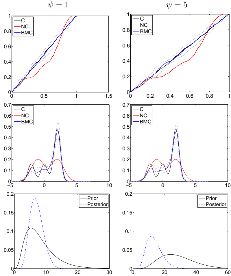
Figure 3: Infinite beta mixture calibrated (BMC), calibrated (C) and non calibrated (NC) combinations for a dataset of 1,000 samples from p_1\mathcal{N}(-2, 0.25) + p_2\mathcal{N}(0, 0.25) + p_3\mathcal{N}(2, 0.25) with \mathbf{p} = (1/5, 1/5, 3/5) . PIT's cdf (top graph) and calibrated pdf (middle graph) of the combination models C (black), NC (red) and BMC (blue) and BMC 99% HPD (gray). Prior (black) and posterior (blue) number of components of the random BMC model (bottom graph).
