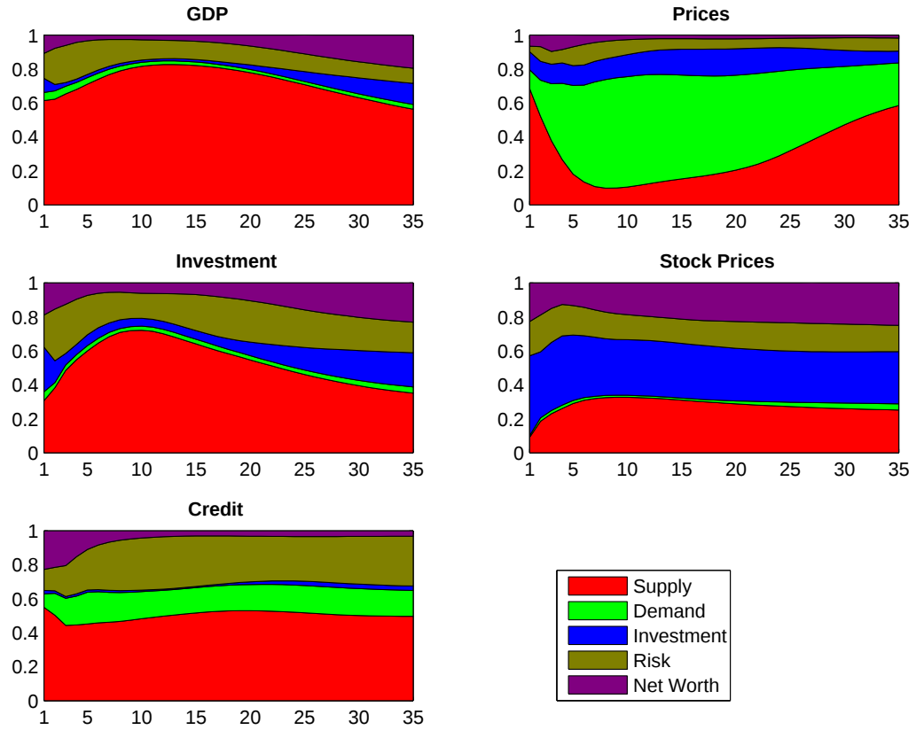
Figure 17: Median forecast error variance decompositions at each horizon for the model including risk and net worth shocks.
