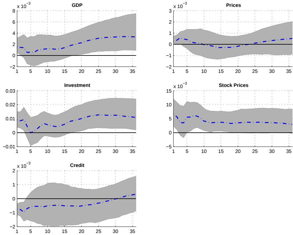
Figure 19: Median impulse responses to a one-standard-deviation net-worth shock for the model including risk and net-worth shocks.
