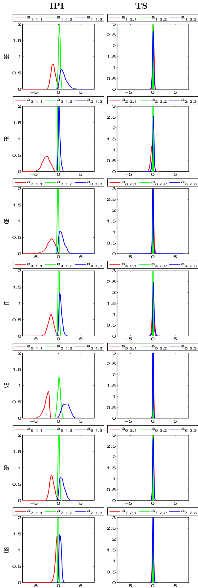
Figure 2: Posterior densities of the Markov-switching intercepts, \gamma_{im} = (a_{i1,m}, a_{i2,m})' , i = 1, \dots, N , m = 1, \dots, M for IPI growth rate and TS.
