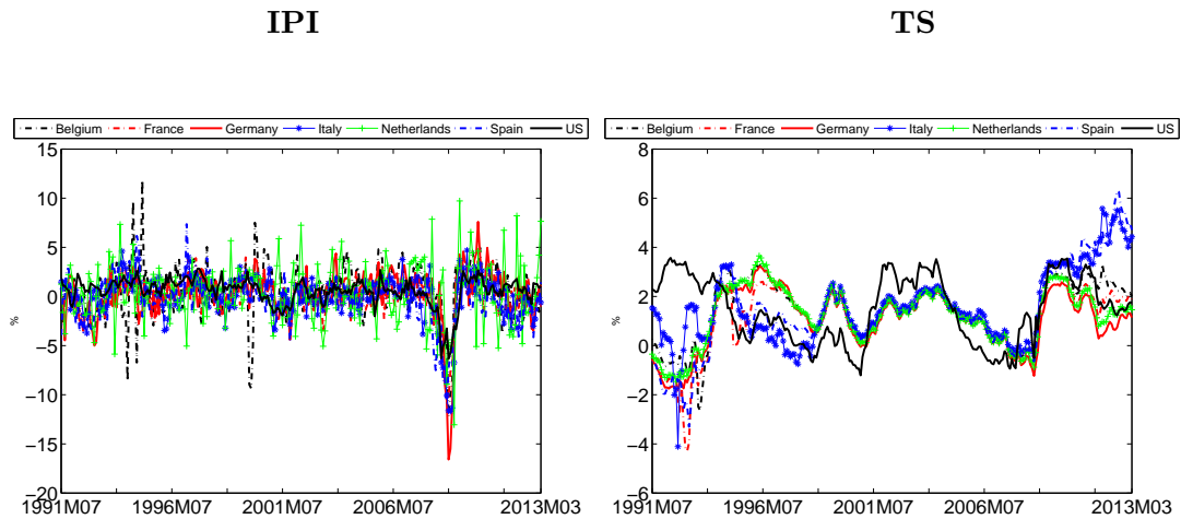
Figure 1: Country-specific endogenous variables: industrial production growth rate (IPI) and term structure (TS).
