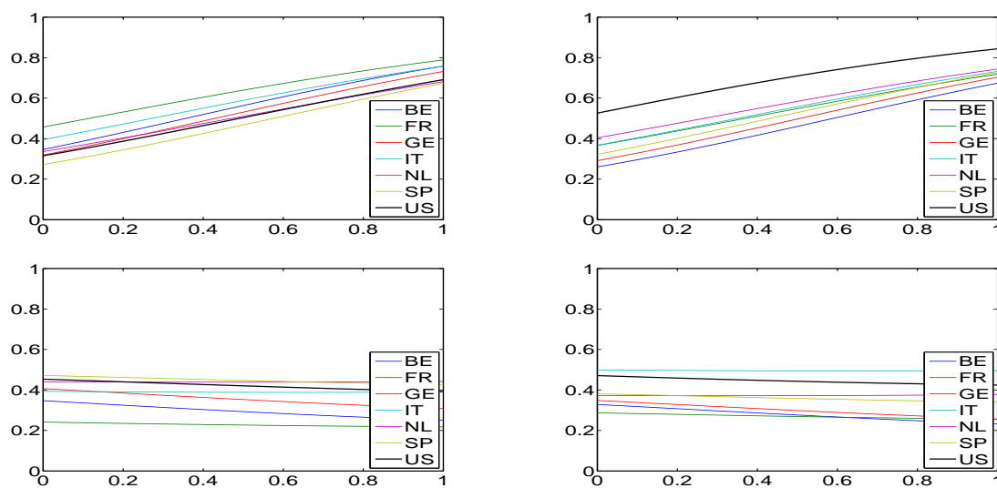
Figure 6: Reaction of the transition probabilities p_{it,11} (first row) and p_{it,12} (second row) to changes in \eta_{1t} , when conditioning on not recession for the US, i.e. s_{7,t} \neq 1 (left column) and recession for the US, i.e. s_{7,t} = 1 , (right column).
