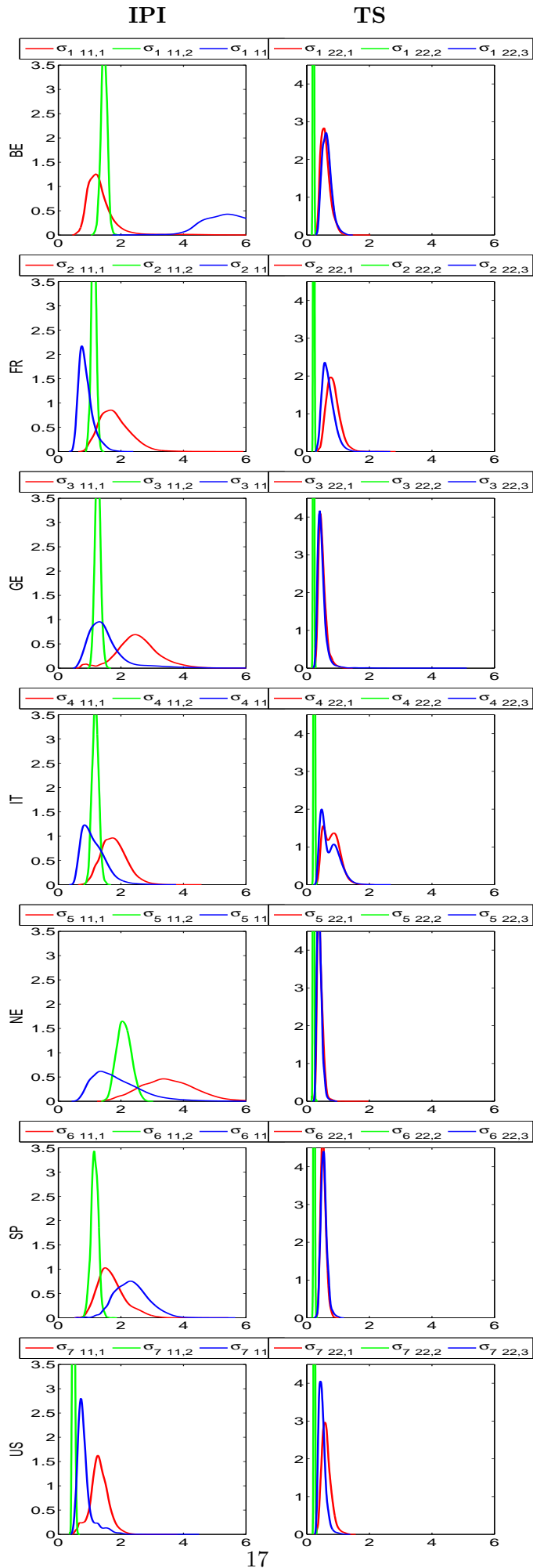
Figure 3: Posterior densities of the Markov-switching volatilities, \sqrt{\sigma_{ijj,m}} , for IPI and TS, with \sigma_{ijj,m} , j = 1, 2 , diagonal elements of \Sigma_{im} , i = 1, \dots, N and m = 1, \dots, M .
