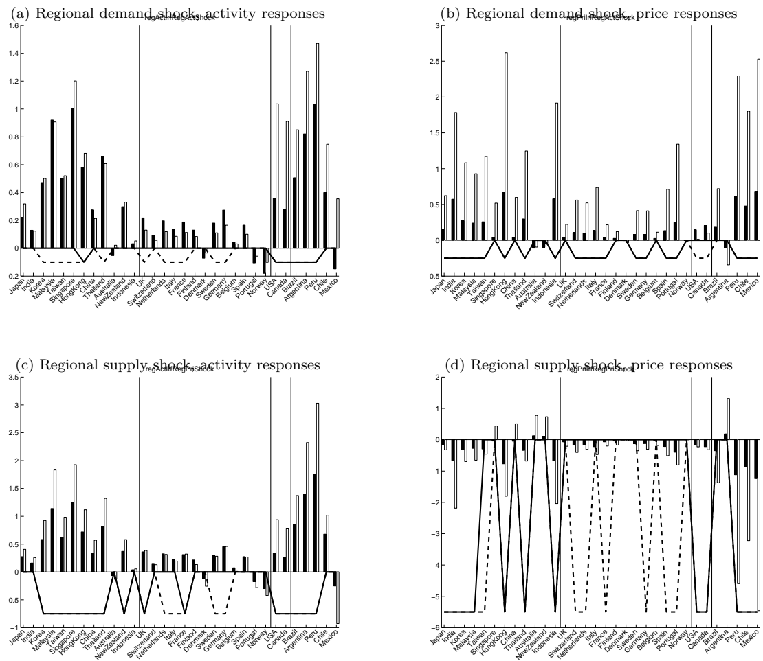
Figure 4: Impulse responses: Regional shocks
