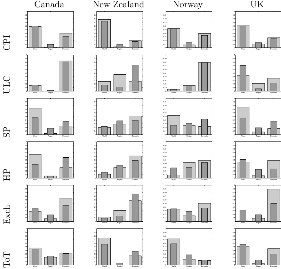
Figure 8: Variance decomposition
