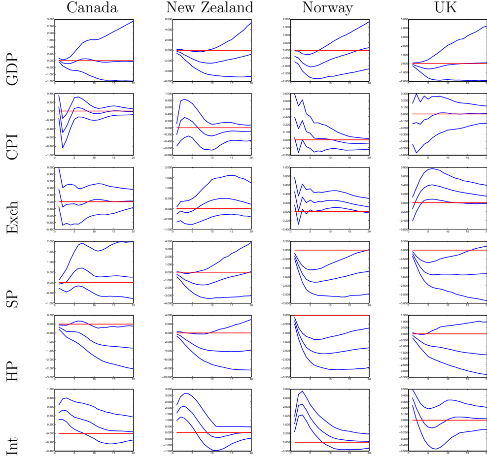
Figure 6: Impulse responses - regional monetary policy shock
