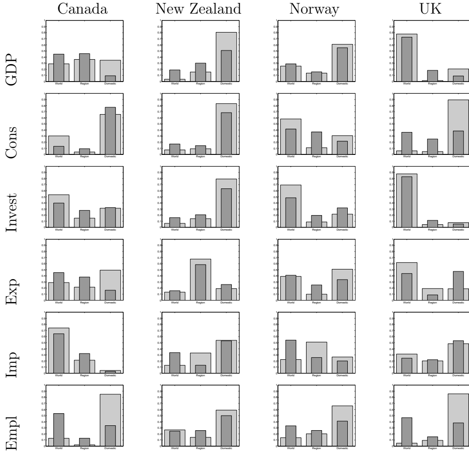
Figure 7: Variance decomposition
