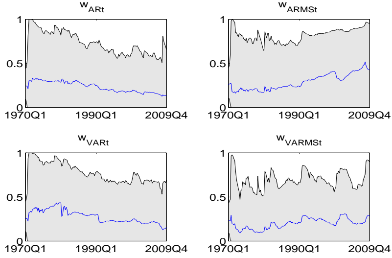
Figure 6: Time-varying weights without learning
