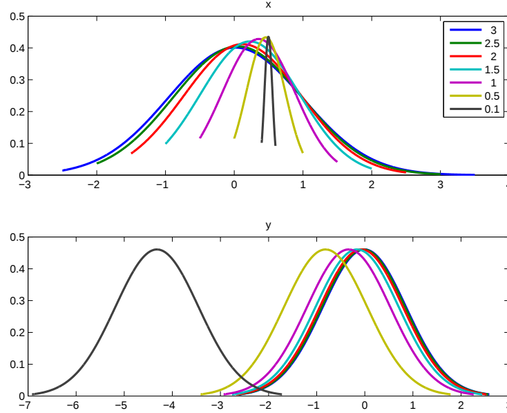
Figure 1: Bivariate normal example
