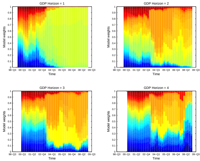
Figure 6: Evolution of GDP score-based weights
