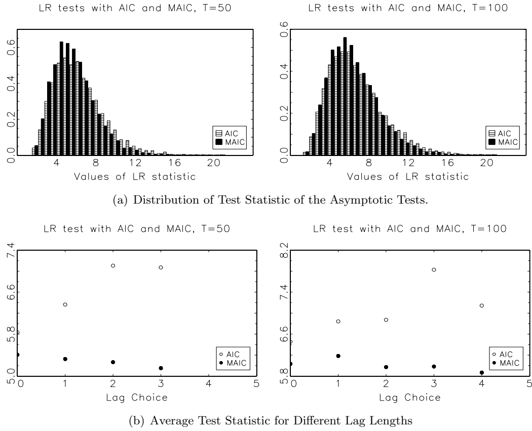
Figure 3: Comparison of the LR test with AIC and MAIC . All graphs refer to the Toda-DGP (7), a_1 = 0.9 ( r = 1 ).
