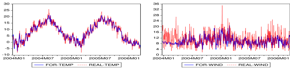
Figure 3: Weather variables: Eastern Denmark
