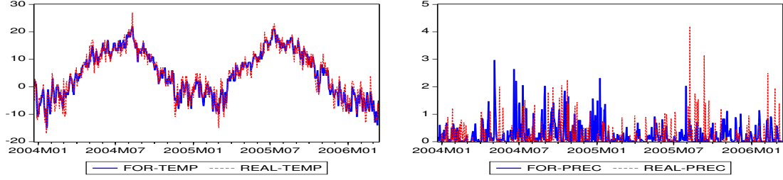
Figure 2: Weather variables: Oslo
