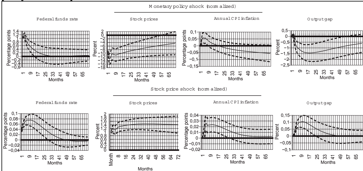
Figure 2: Structural identification: Impulse response due to the identified monetary policy and stock price shock.
