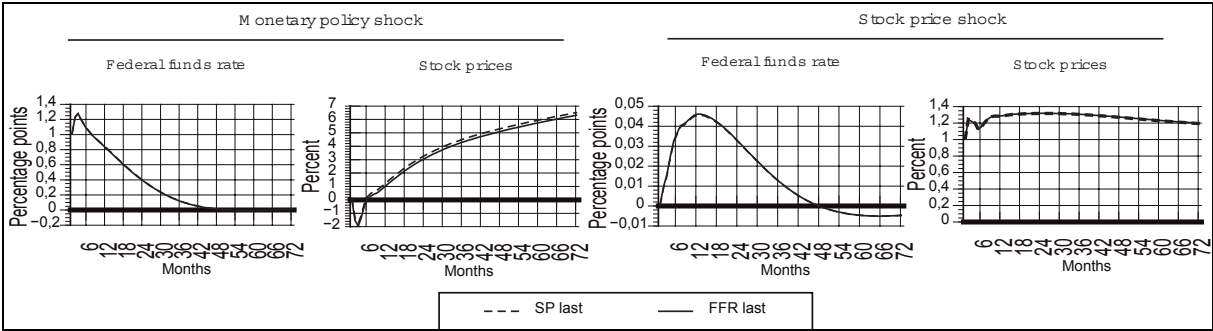
Figure 1: Cholesky decomposition: Impulse responses due to monetary policy and stock price shocks.
