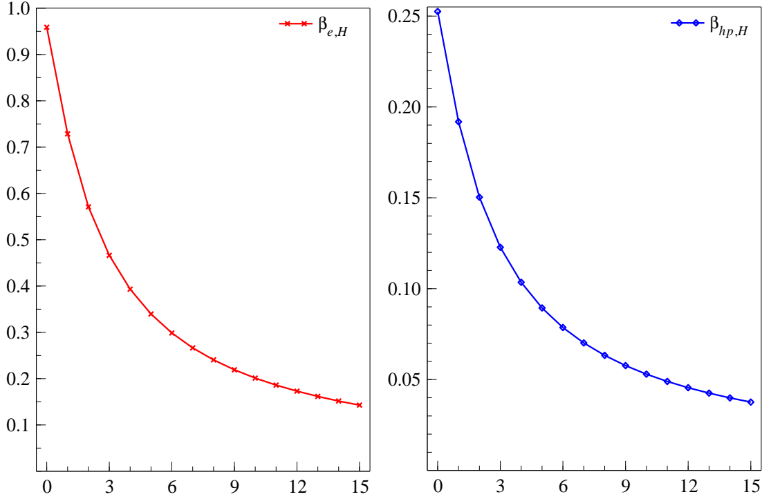
Figure 4: Left: Initial interest rate responses to the nominal exchange rate shock (in percentage points) implied by different policy horizons (horizontal axes), \beta_{e,H} . Right: Left: Initial interest rate responses to the house price shock (in percentage points) implied by different policy horizons, \beta_{hp,H} .
