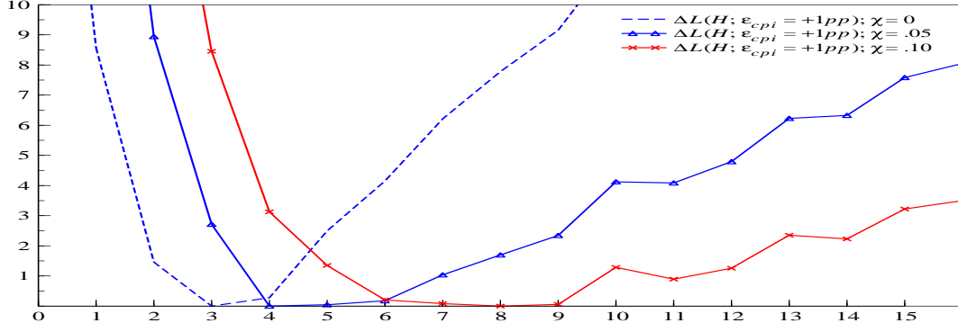
Figure 16: Plots of the relative loss function defined by different \chi values against different policy horizons in the case of the the supply shock. The policy horizon is optimal when \Delta L(.) = 0 and the relative loss is measured in %.
