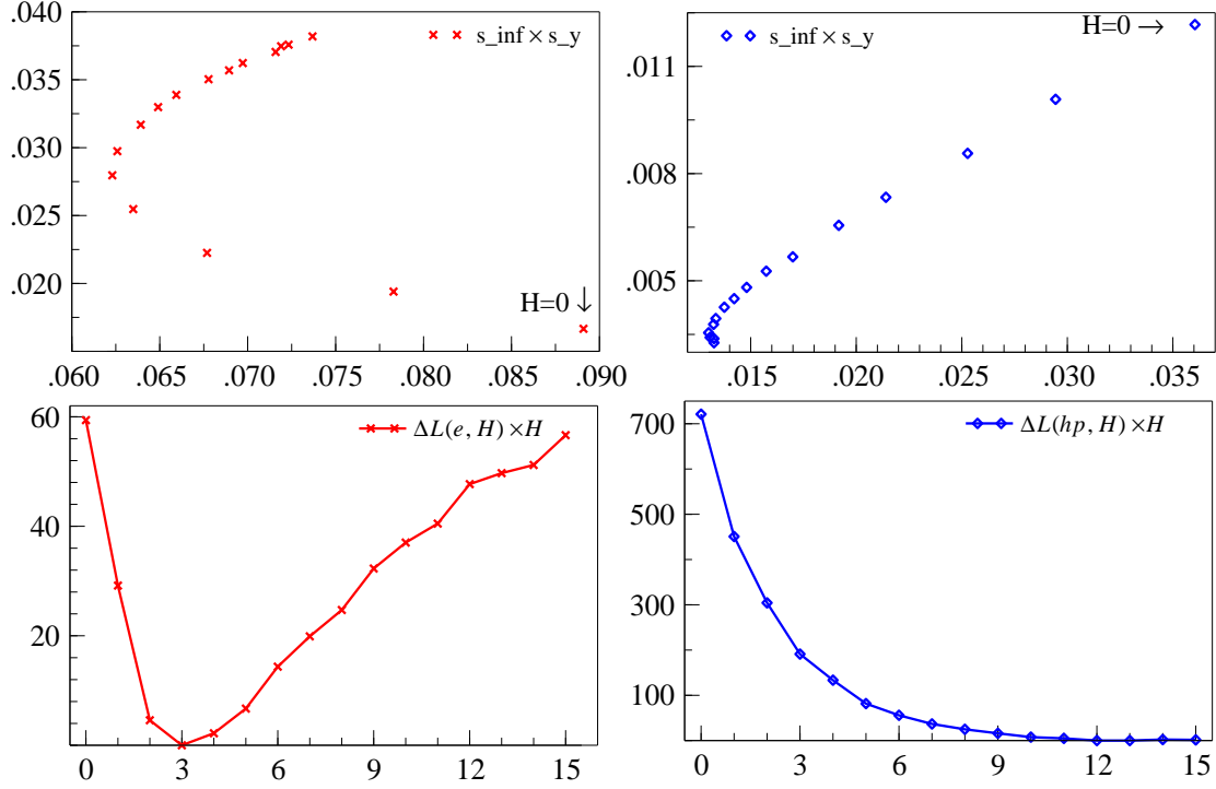
Figure 5: Top: Performance of the policy rules associated with different policy horizons in the face of the exchange rate shock (left-hand side) and the house price shock (right-hand side), respectively. The policy rules are associated with policy horizons ( H s) in the range of 0-15 quarters. See Figure 3 for more details.
