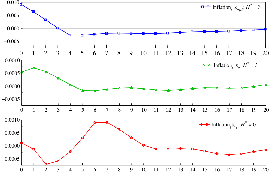
Figure 6: Convergence of inflation to its target rate in response to different shocks under the corresponding optimal policy rules, which are represented by the optimal policy horizons H^* . Optimal target horizons are suggested by the first 'touch down' of inflation to its target rate, indicated by zero on the vertical axes. The horizontal axes indicate the time periods in quarters.
