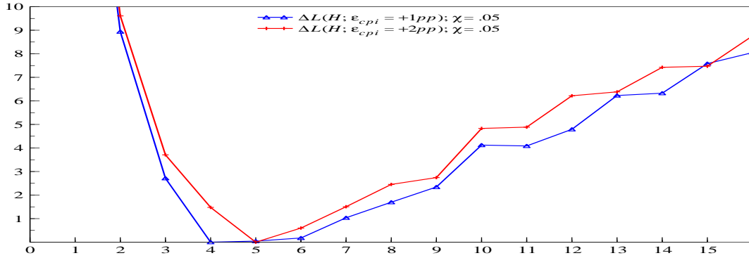
Figure 9: Plots of the values of the relative loss function ( \Delta L(.) ) (in %) at different policy horizons in the case of supply shocks of different sizes. The loss function has been modified to incorporate concern for interest rate volatility which is measured by \chi and its value has been set to 0.05. The policy horizon is optimal when \Delta L(.) = 0 .
