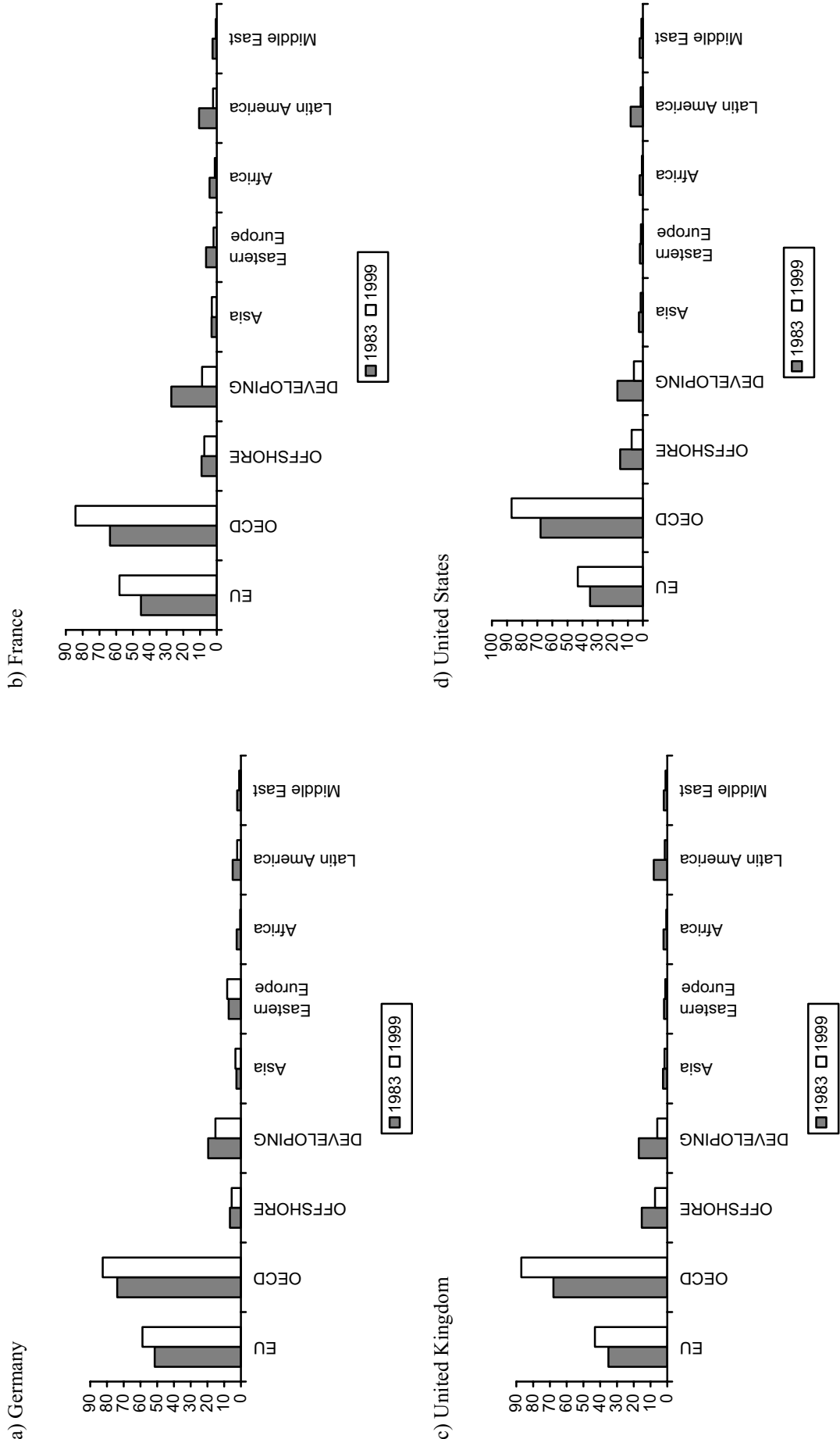
Figure 1 — Regional Structure of Foreign Assets, Locational Data
