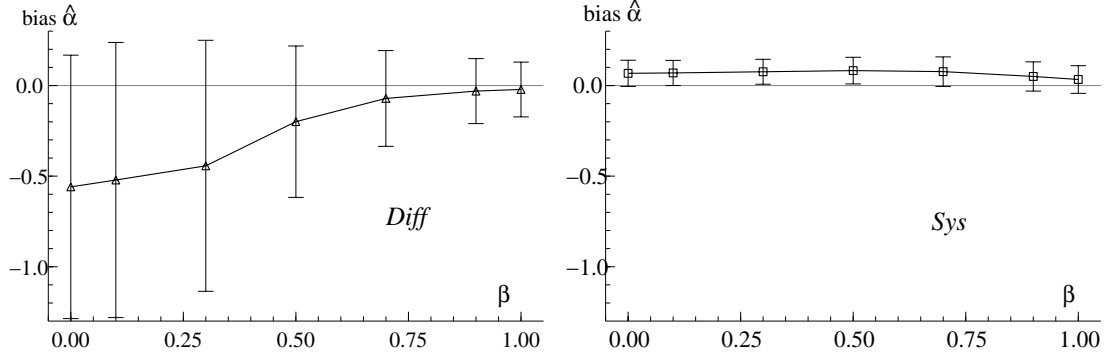
Figure 6: Mean bias of \hat{\alpha} , M = 1000, \alpha = 0.9, \rho = 0.8, \sigma_e^2 = 0.9 ; bars are twice the MCSD; \beta = 0, 0.1, 0.3, 0.5, 0.7, 0.9, 1 .
