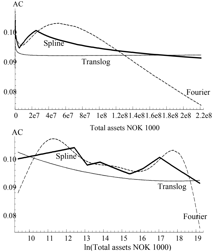
Figure 2.2: Average costs plotted against total assets for different cost function specifications, upper panel. Average costs plotted against ln of total assets, lower panel.
