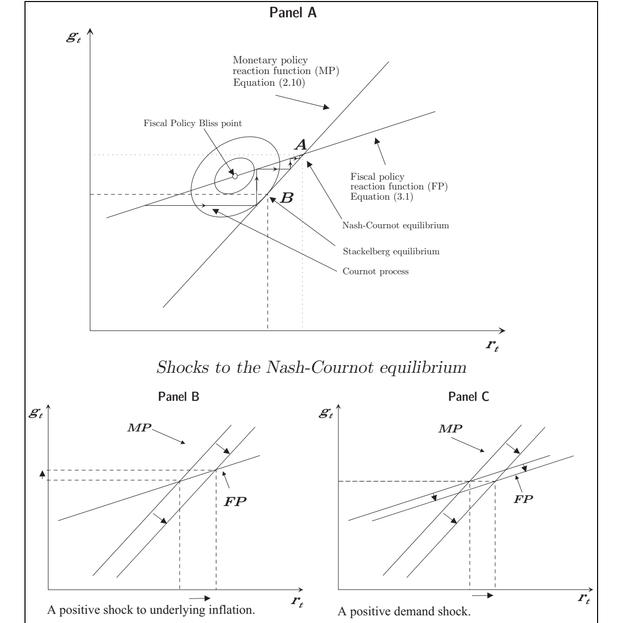
Figure 3.1: An illustration of the two equilibria
